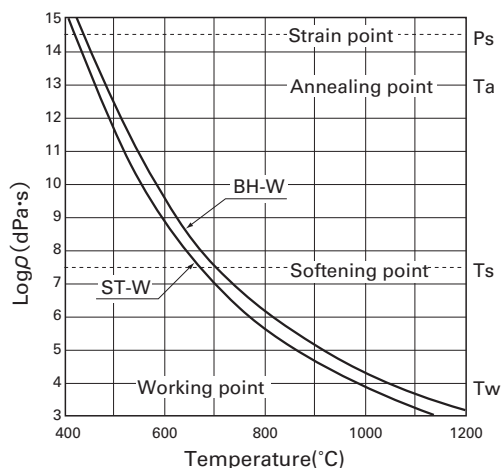
Fig. 3 Viscosity
