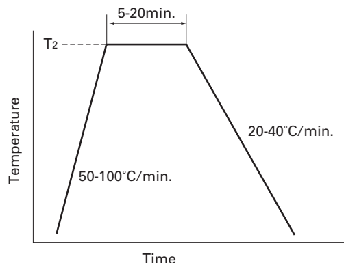
Fig. 2 Sealing profile
