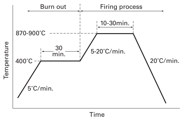
Fig. 1 Firing profile
